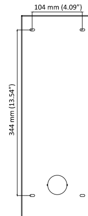
Rear View
